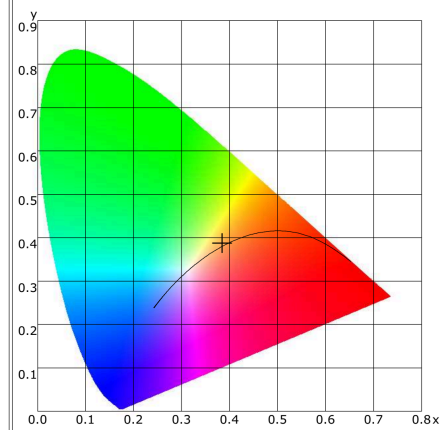
CIE1931
