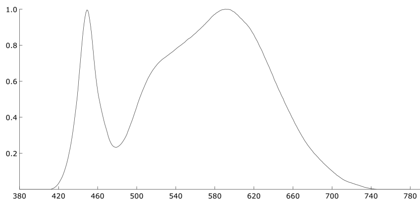
Spectrogram
