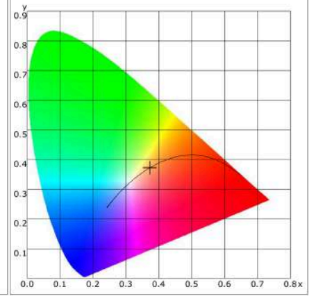
CIE1931
