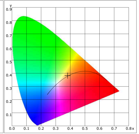
CIE1931
