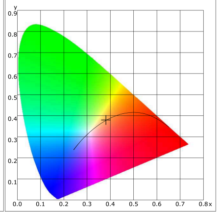
CIE1931
